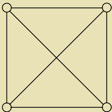
(a) K_4
